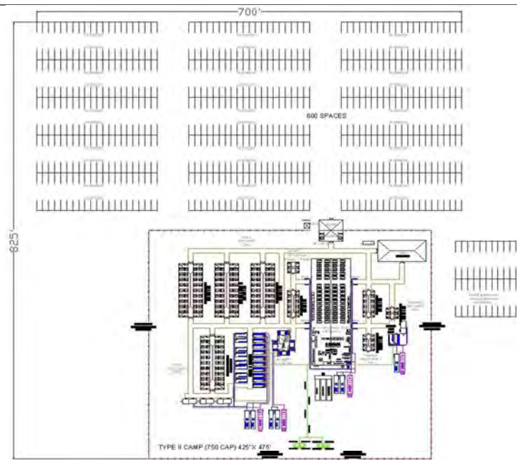
Figure 3: TYPICAL - TYPE II BASE CAMP - 750 PERSONS
