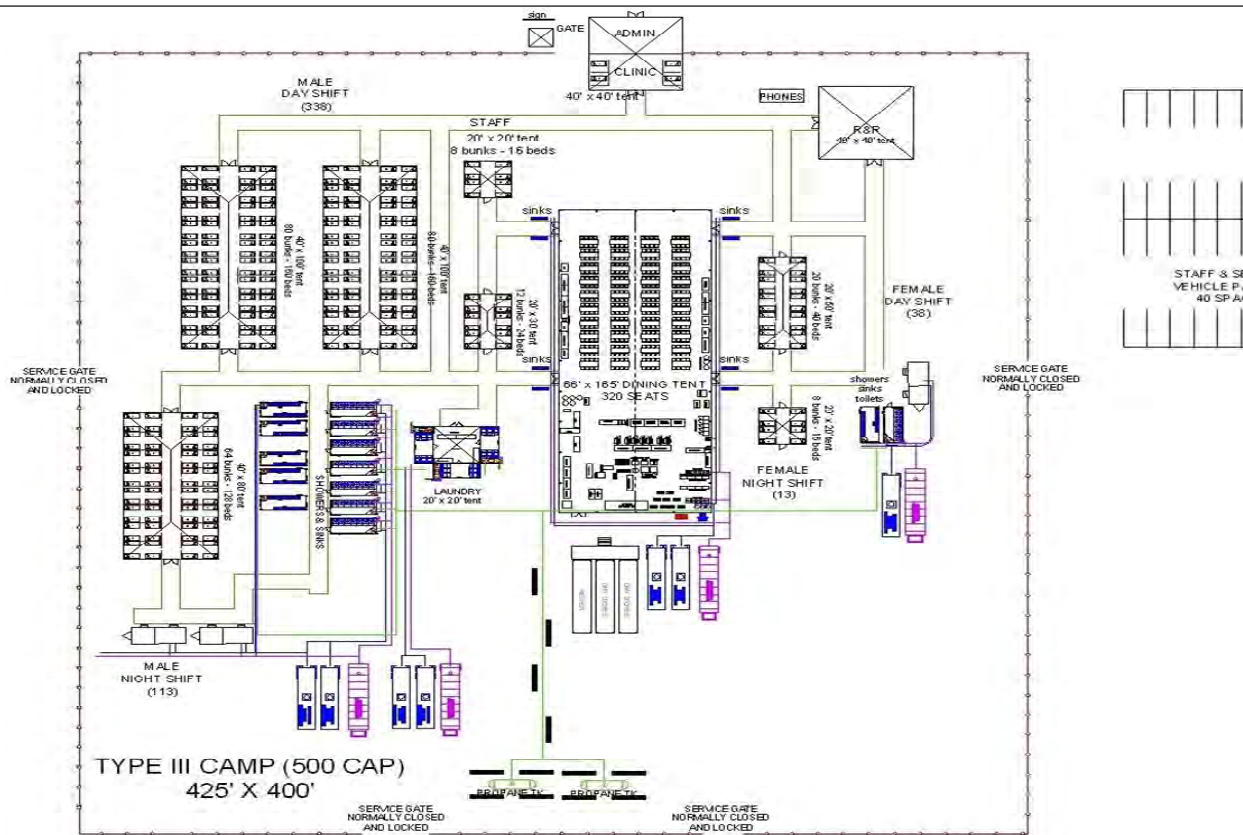
Figure 6: TYPICAL - TYPE III BASE CAMP - 500 PERSONS
