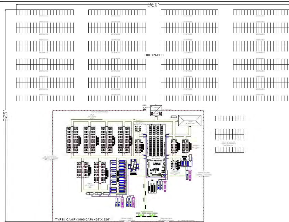
Figure 9: TYPICAL - TYPE IV EMERGENCY SHELTER - 1000 PERSONS
