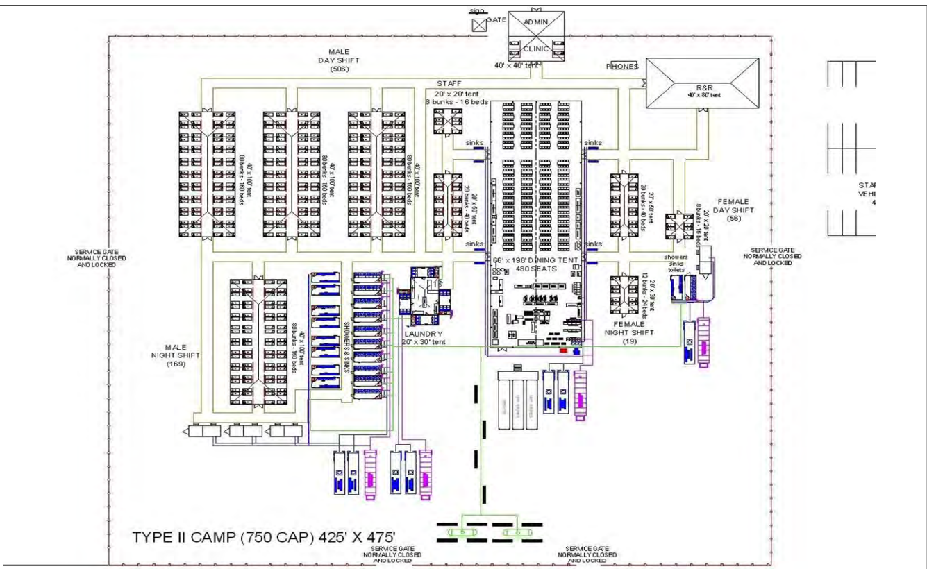
Figure 4: TYPICAL - TYPE II BASE CAMP - 750 PERSONS
