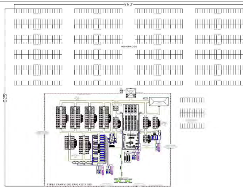
Figure 1: TYPICAL - TYPE I BASE CAMP - 1000 PERSONS
