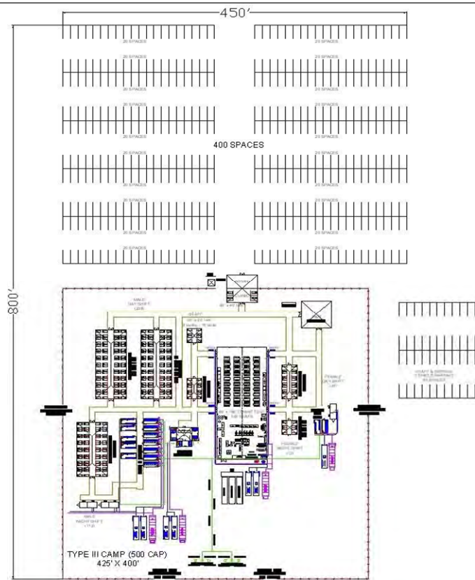
Figure 5: TYPICAL - TYPE III BASE CAMP - 500 PERSONS
