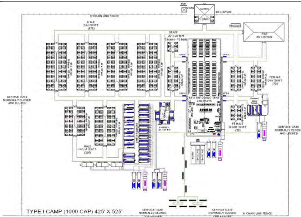
Figure 2: TYPICAL - TYPE I BASE CAMP - 1000 PERSONS
