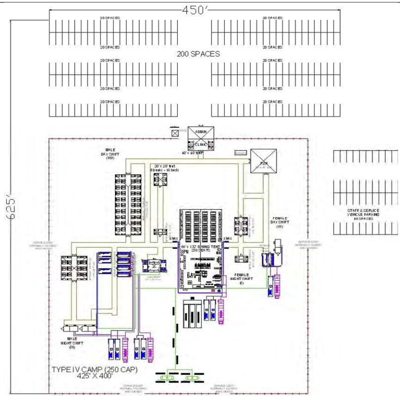
Figure 7: TYPICAL - TYPE IV BASE CAMP - 250 PERSONS
