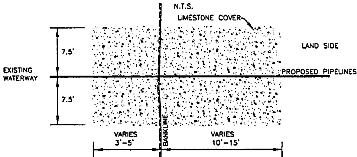
TYPICAL PLAN
