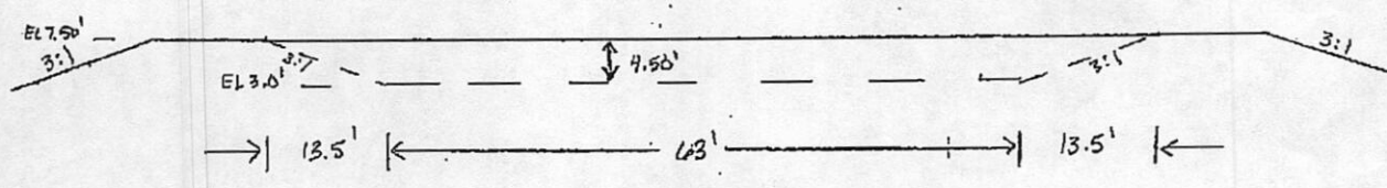
SECTION C-C
