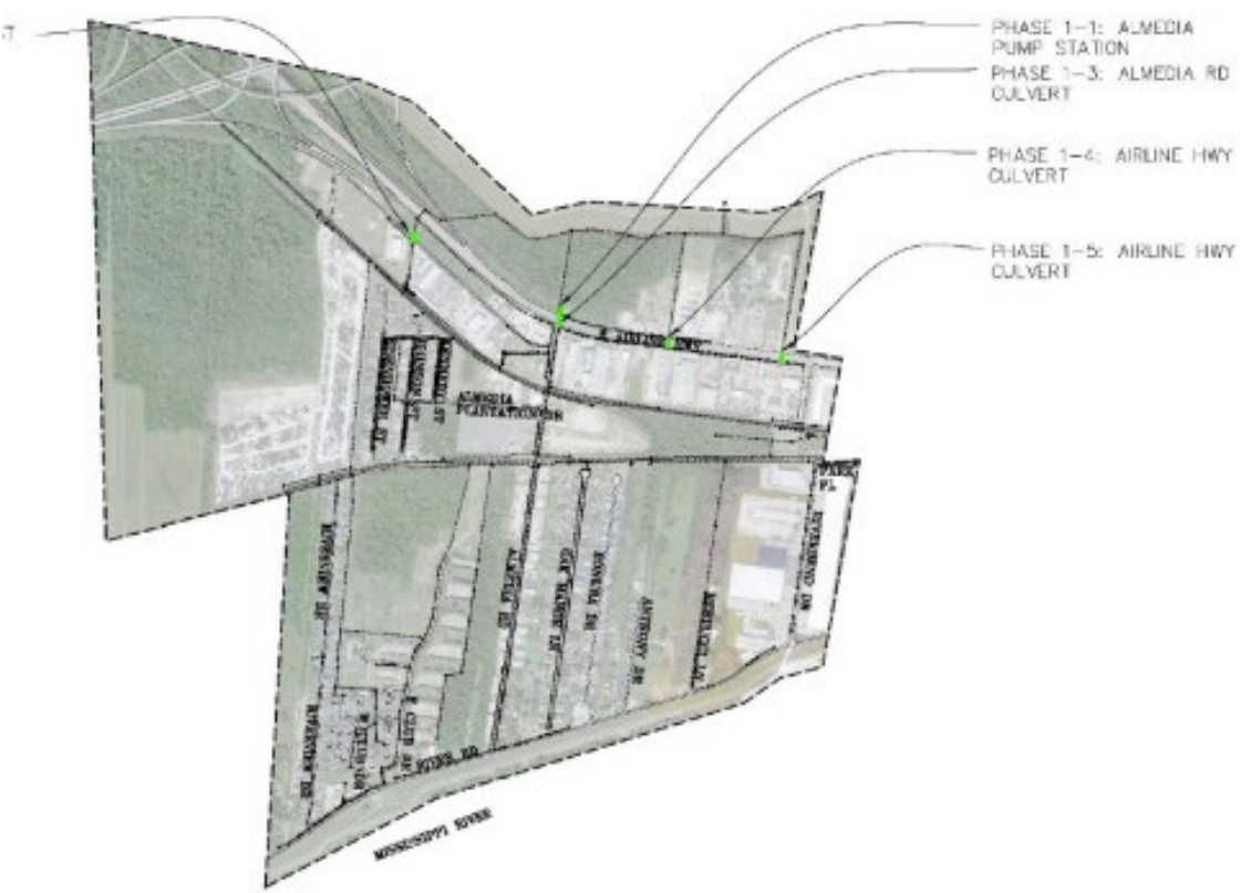
TURTLE POND PROGRAM - PHASE 1 IMPROVEMENTS 25-YEAR CRITERIA WITH SELECTED 100-YEAR IMPROVEMENTS
