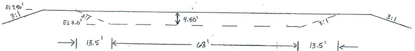
SECTION C-C
