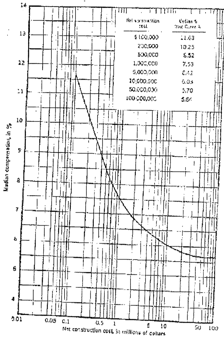
FIG. 1.—CURVE A. MEDIAN COMPENSATION FOR BASIC SERVICES EXPRESSED AS A PERCENTAGE OF NET CONSTRUCTION COST FOR PROJECTS OF ABOVE-AVERAGE COMPLEXITY (1950)
