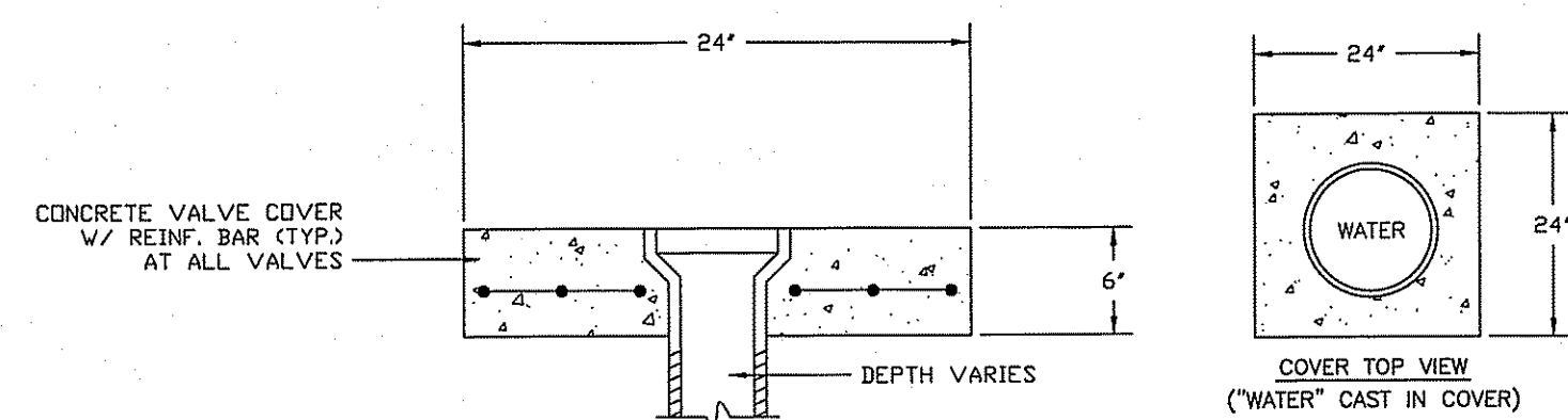
VALVE PAD DETAIL
