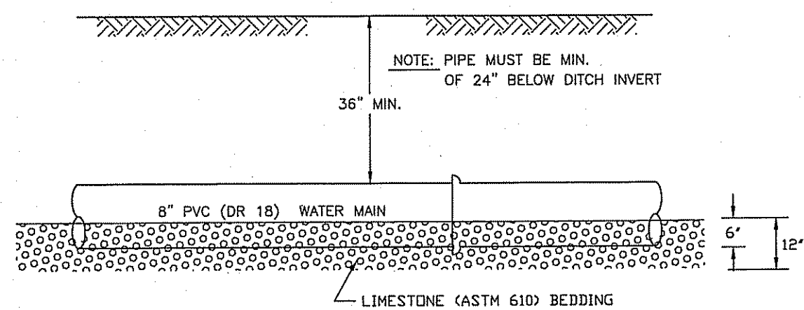
PIPE LAYING PROFILE
