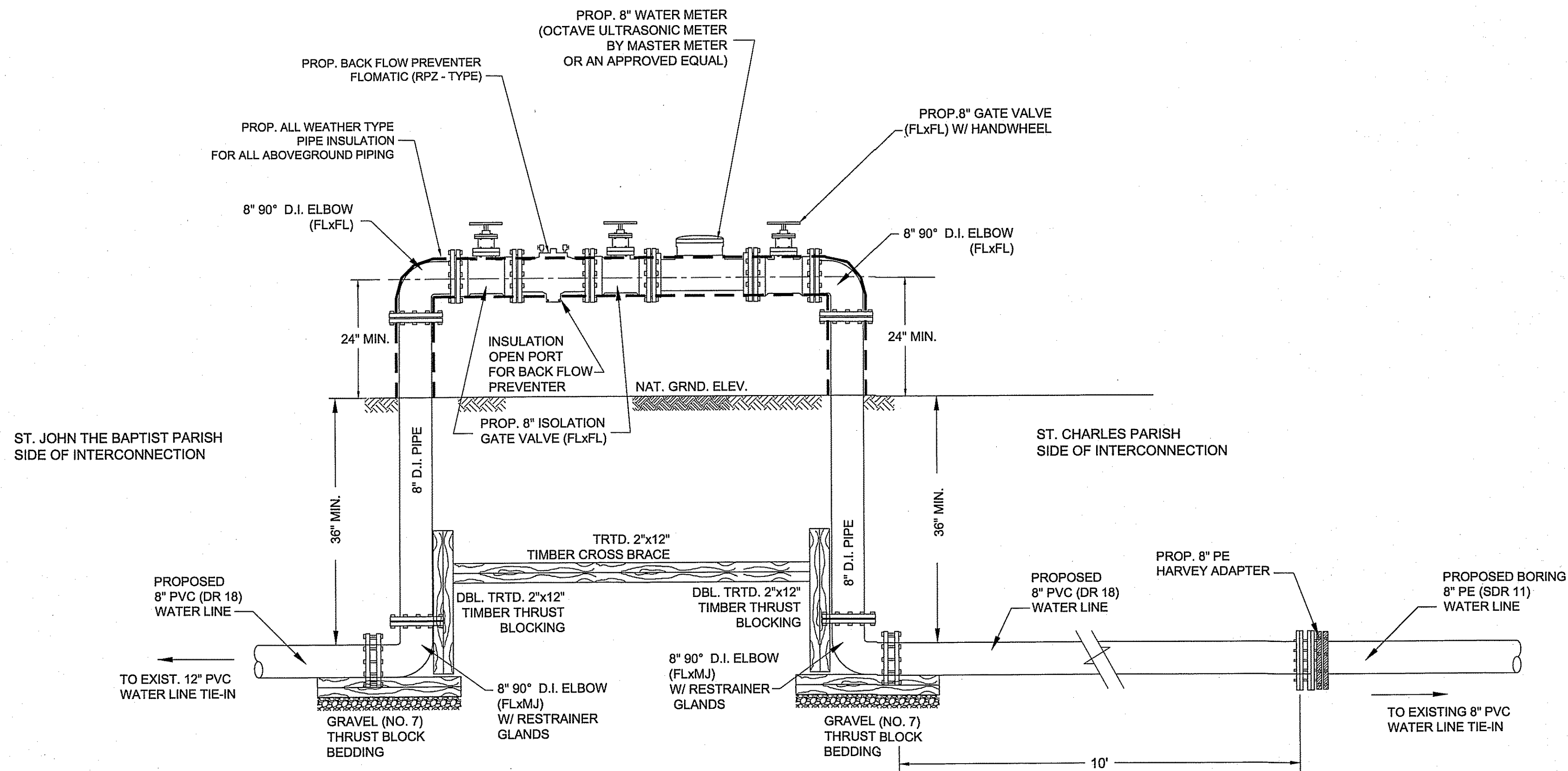
PROPOSED METER ASSEMBLY DETAIL
