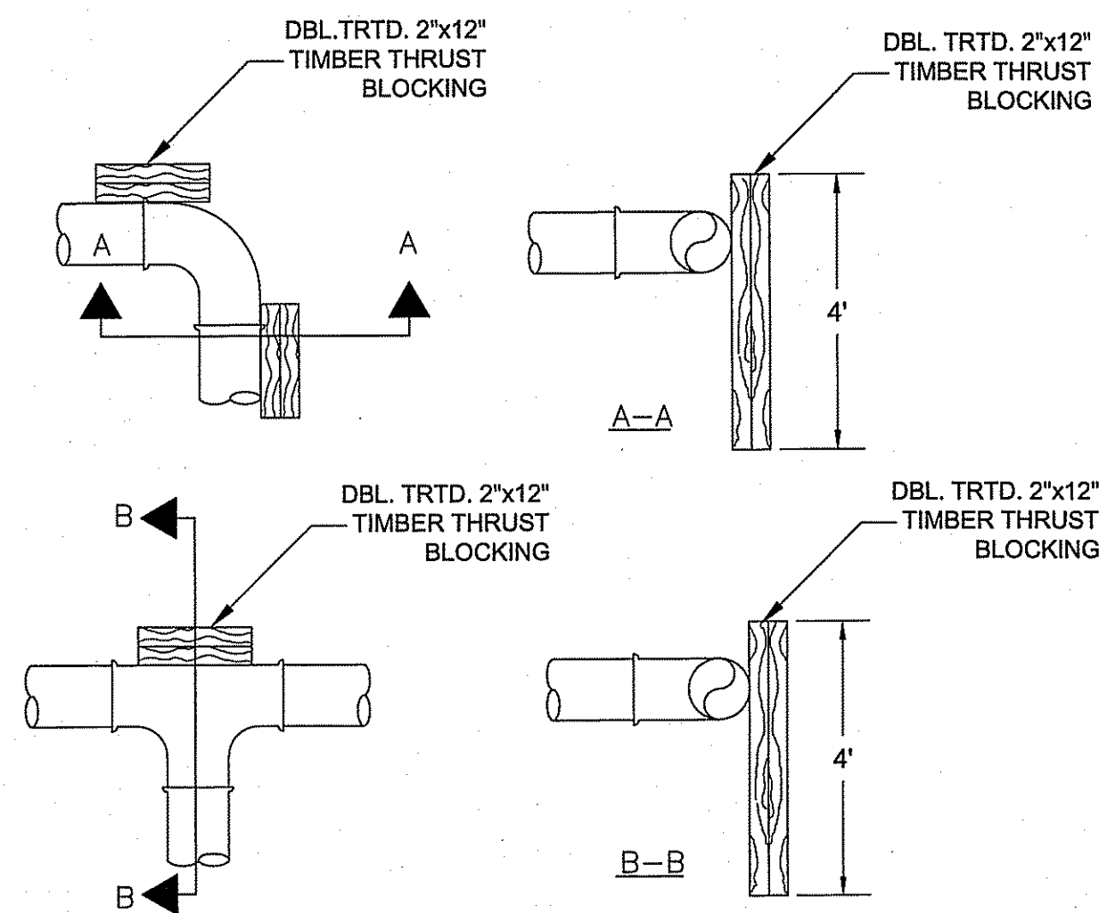
TIMBER BLOCKING TYP. DETAIL
