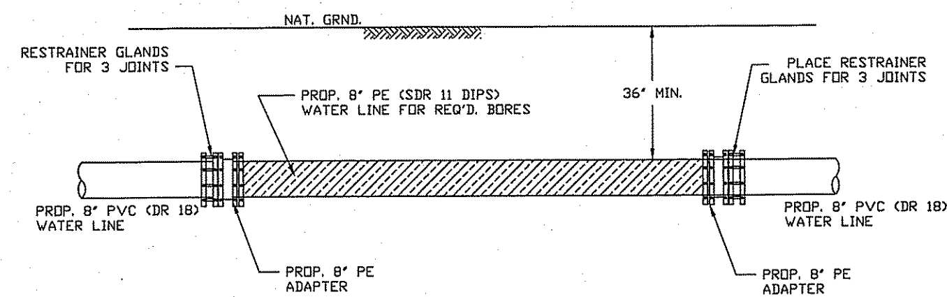
POLYETHYLENE BORE DETAIL (TYP.)
