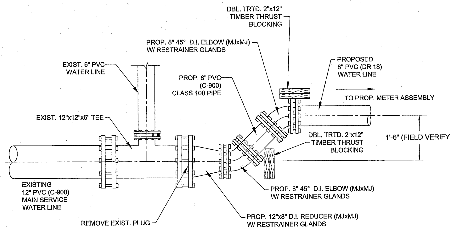
ST. JOHN PARISH WATER LINE TIE-IN DETAIL
