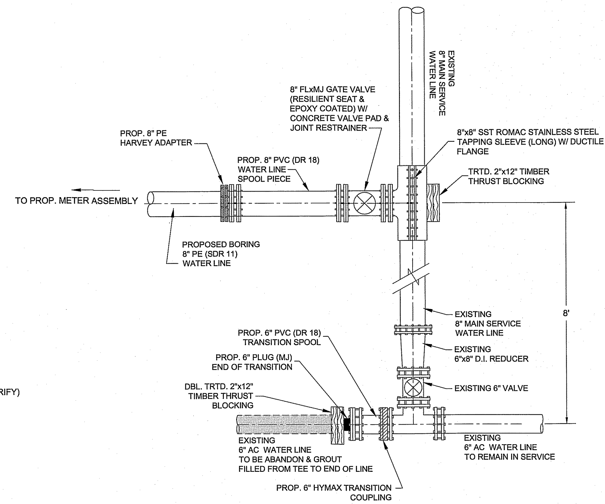
ST. CHARLES PARISH WATER LINE TIE-IN DETAIL
