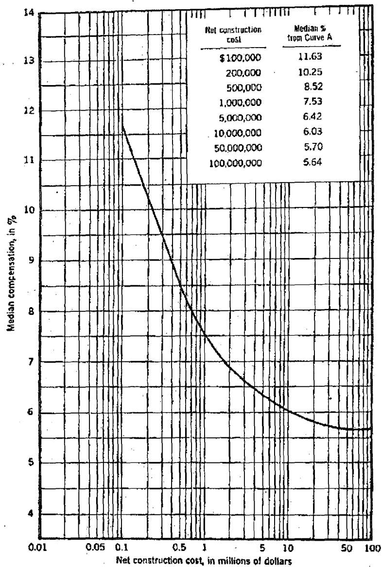
FIG. 1.—CURVE A. MEDIAN COMPENSATION FOR BASIC SERVICES EXPRESSED AS A PERCENTAGE OF NET CONSTRUCTION COST FOR PROJECTS OF ABOVE-AVERAGE COMPLEXITY (1988)
