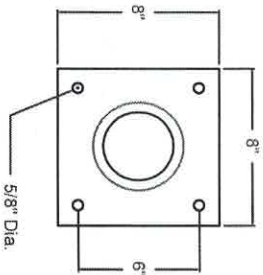
Base Plate Detail Mat: 3/8" Plate CS
